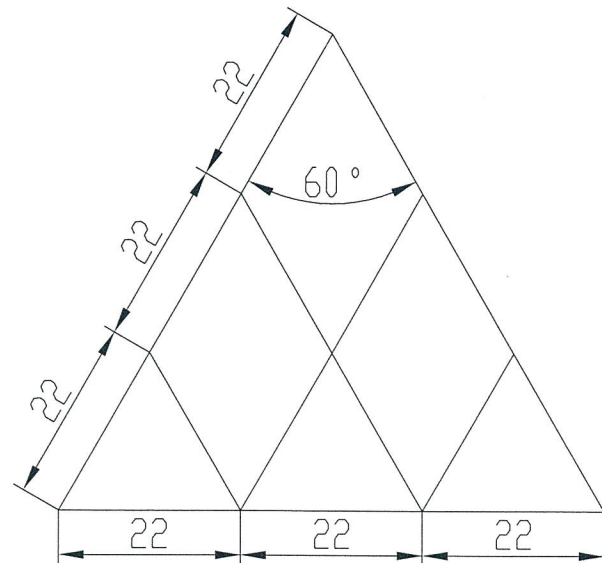
DETAIL DRAWING OF TUBE PITCH 孔距详图
